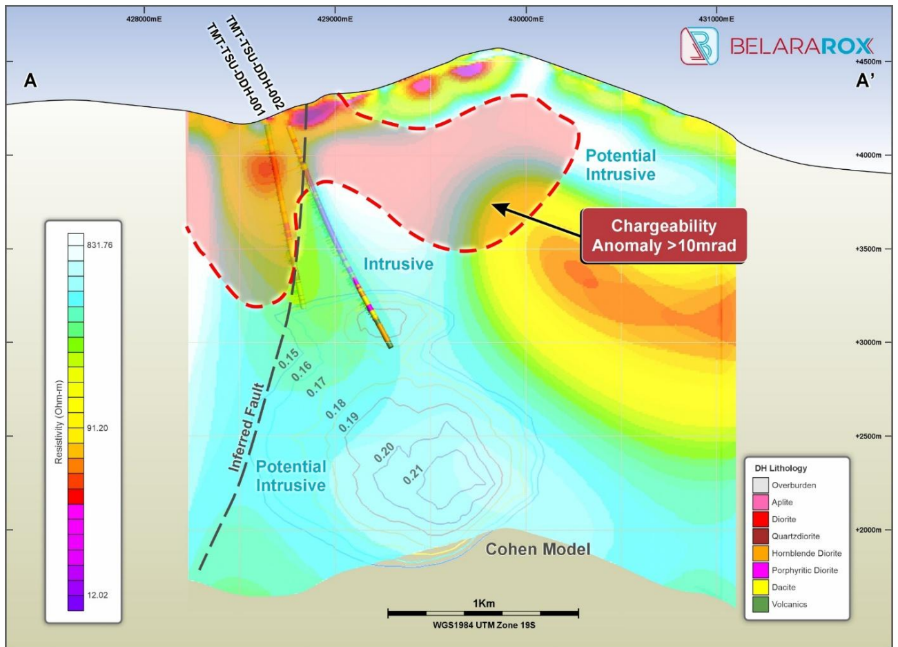
Figure 4. Cross-section A-A' (refer to Figure 3 for section location in plan view) of the Tambo South Target showing drill holes TMT-TSU-DDH-001 and TMT-TSU-DDH-002 from the 2025 field season drilling 5 , chargeability and resistivity anomalies from the recently completed MT/IP survey and geochemical anomaly. Note: The numbers on the iso surfaces represent probability scores (0.0-1.00) of the geochemical models at Toro South matching with the reference metal-zoning models from Cohen (2011). Values over 0.15 are considered 'significant', with a maximum score of 1.00, which corresponds to a 100% match.
