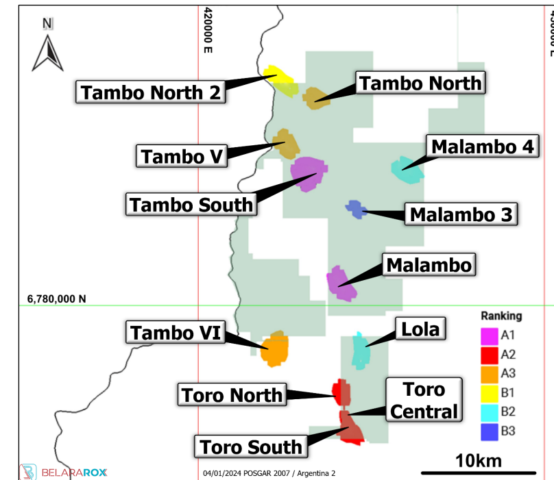
Targets from ASTER and SENTINEL 2 interpretation
